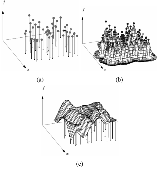
Figure 3: Data values \{\mathbf{x}_i, h_i\}_1^M (Figure 3a), the RBF collocation functions (Figure 3b), the resulting interpolant (Figure 3c). (From [FW09]).
