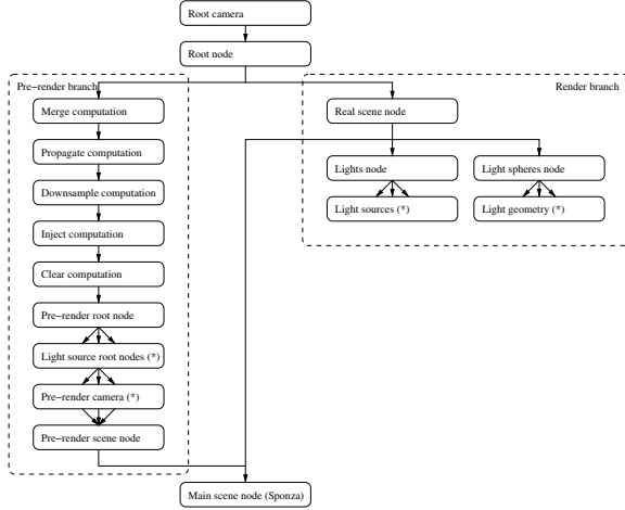
Figure 3: Diagram showing the structure of the scene graph used in the real-time implementation. Non-essential branches have been omitted. Nodes marked with a star (*) and diverging incoming arrows, may exist in multiple copies for each parent node.
