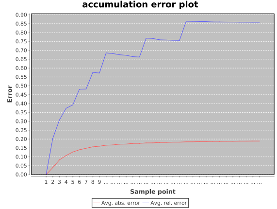
Figure 8: The errors measured after each iteration during a simulation. Both the average absolute errors and the average relative errors are presented.
