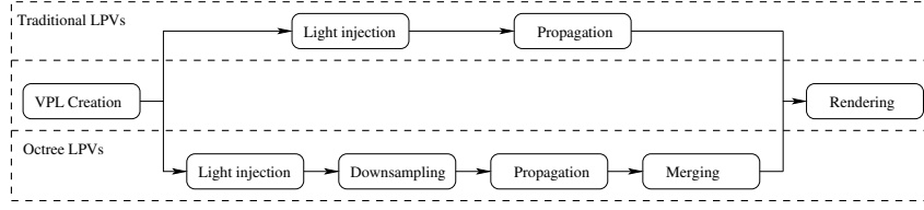
Figure 1: An overview of the steps included in the octree based and the traditional light propagation volumes technique. The steps are divided into those that are the same for both techniques and those that need to be implemented specifically for one particular technique.
