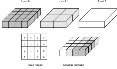
Figure 2: A two dimensional slice of a flattened index volume, three levels of a full octree and the resulting sampling.
